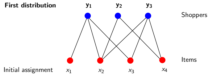
Figure 5: Bipartite network: distribute relevance of each item among its buyers according to how many shoppers bought the item. E.g if relevance is distributed evenly, then y_1 = x_1 + x_2/3 + x_3/2 .
