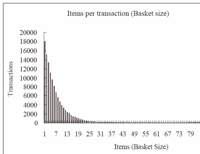
Figure 2: Data Sparsity: Items per transaction.
