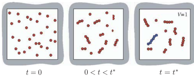
FIG. 1. Homogeneous self-assembly and growth in a closed unit volume initiated with M = 30 free monomers. At a specific intermediate time 0 < t < t^* in this depicted realization, there are six free monomers, four dimers, four trimers, and one cluster of size four. For each realization of this process, there will be a specific time t^* at which a maximum cluster of size N = 6 in this example is first formed (blue cluster).
