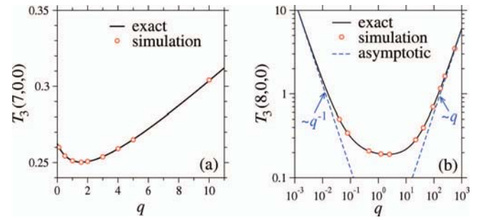
FIG. 4. Mean first assembly times for M = 7 and N = 3 in panel (a) and M = 8 and N = 3 in panel (b). Exact results derived in Eq. (12) are plotted as black solid lines, while red circles are obtained by averaging over 10^5 KMC trajectories. The dashed blue line shows the q \rightarrow 0 approximation in Eq. (18) and the q \rightarrow \infty approximation in Eq. (23).
