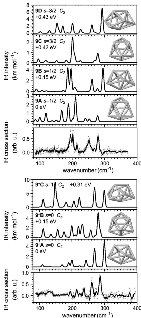
FIG. 6. Vibrational spectra of Nb 9 (upper panel) and Nb 9 + (lower panel).
