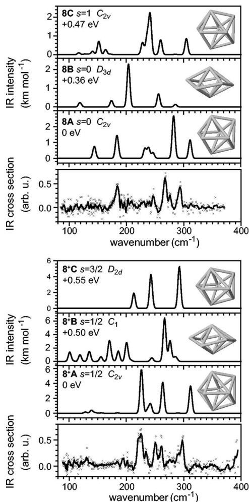
FIG. 5. Vibrational spectra of Nb 8 (upper panel) and Nb 8 + (lower panel).
